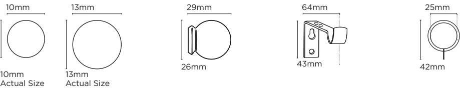
Pole Diameter
